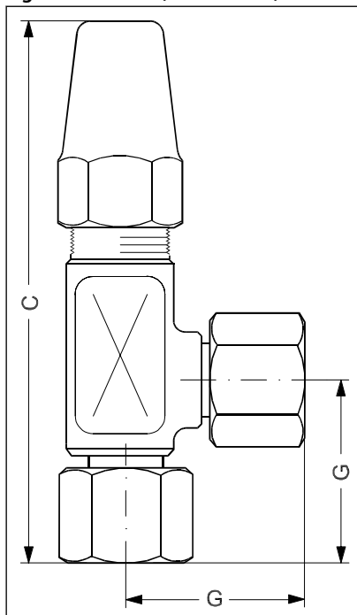
Figure 4: SNV-ST (Manometer)
